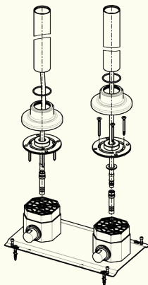
Fixing diagram
